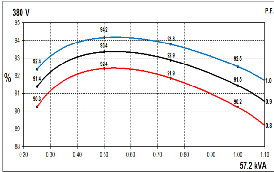
50Hz Curves
