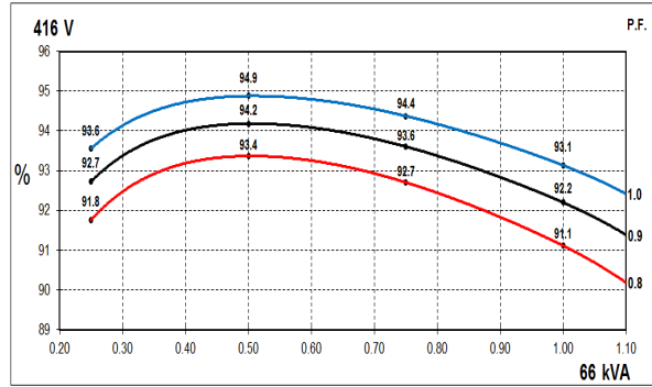
60Hz Curves
